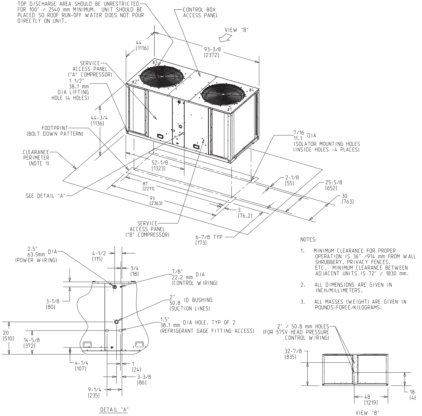
Figure DD-8 – TTA200F Condensing Unit
